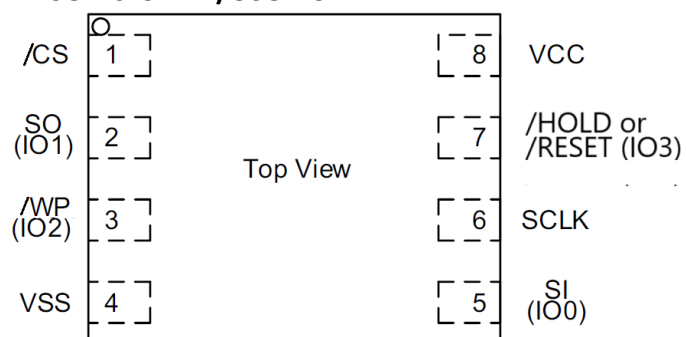
Figure 1b. 8-pad WSON 6x5-mm/USON 3x4-mm
