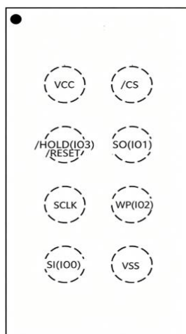
Figure 1c. Pad Assignments, 8Ball WLCSP (Top View)
